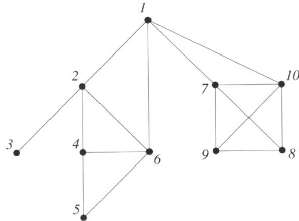
Figure 7.4 A DFS for an undirected graph.
