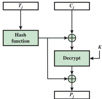
(a) Decryption
