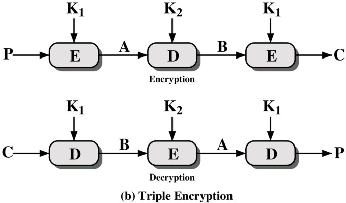
Figure 6.1 Multiple Encryption
